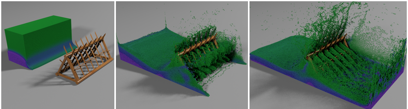
Figure 13: 3D Dambreak with a complex obstacle. The pressure field is color coded and the projection-based solver takes 8.99s per timestep on average.
