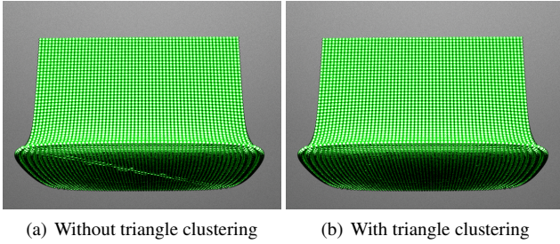
Figure 5: (a) Without triangle clustering, discontinuous artifacts may arise between two adjacent triangles; (b) With triangle clustering, the discontinuity is removed.
