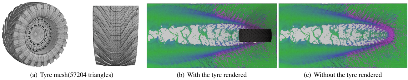
Figure 12: A one-way coupling example between a tyre and a thin layer of water. Velocities are color coded and the projection-based method takes 9.75s per timestep on average.
