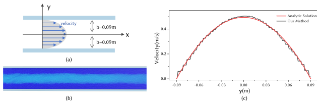
Fig. 15. Poiseuille flow. (a) Schematic of the two-dimensional Poiseuille flow; (b) Steady-state flow (far from the inlet) simulated by our unified method. The particle color is coded by particle velocity. The time step is 0.001s, the particle spacing dx is 0.005m , \lambda = 1.0 , \mu = 0 , \kappa = 1.0 , \gamma = 0 ; (c) Comparison between our method and the analytical solution. The analytical solution refers to [Takeda et al. 1994], i.e. \mathbf{v}(y) = \alpha(1 - y^2/b^2) , where \alpha is the maximum centerline velocity, and b is the channel half-width. The numerical velocity distribution is sampled along the y -axis under steady-state conditions.
