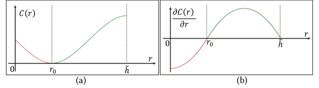
Fig. 4. Pairwise potential energy for surface tension (a) and its first derivative with respect to inter-particle distance (b). \tilde{h} is the radius of neighborhood. Similar to van der Waals interactions, particles experience repulsion at short ranges (red region of the potential curve) to resist compression and attraction at longer ranges (green region). The potential energy is minimized when the interparticle distance matches the equilibrium spacing ( r_0 ).
