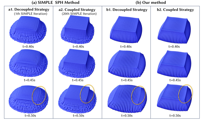
Fig. 8. Viscosity fluids. (a1) SIMPLE SPH method [Liu et al. 2022] with a single SIMPLE iteration, decoupling viscosity [Weiler et al. 2018] and incompressibility [Kang and Sagong 2014]; (a2) SIMPLE SPH method [Liu et al. 2022] with 20 SIMPLE iterations to couple viscosity and incompressibility; (b1) Our semi-implicit variational method with decoupled treatment of viscosity and incompressibility; (b2) Our unified method with strong coupling between viscosity and incompressibility.
