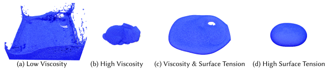
Fig. 5. Different fluids. (a) Low viscosity fluid ( \kappa = 1, \lambda = 0.2, \mu = 0.01, \gamma = 0.01 ); (b) High viscosity fluid ( \kappa = 1, \lambda = 200, \mu = 1, \gamma = 0.01 ); (c) Fluid with moderate viscosity and surface tension ( \kappa = 1, \lambda = 40, \mu = 1, \gamma = 200 ); (d) High surface tension fluid ( \kappa = 1, \lambda = 0.2, \mu = 0.01, \gamma = 1000 ).
