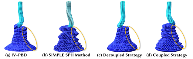
Fig. 9. Coiling effects of viscous fluids. (a) Implicit viscosity [Weiler et al. 2018] combined with PBF [Macklin and Müller 2013]; (b) SIMPLE SPH method [Liu et al. 2022] with 5 SIMPLE iterations to couple viscosity [Weiler et al. 2018] and incompressibility [Nair and Tomar 2014]; (c) Our semi-implicit variational method with decoupled treatment of viscosity and incompressibility; (d) Our unified method with strong coupling between viscosity and incompressibility.
