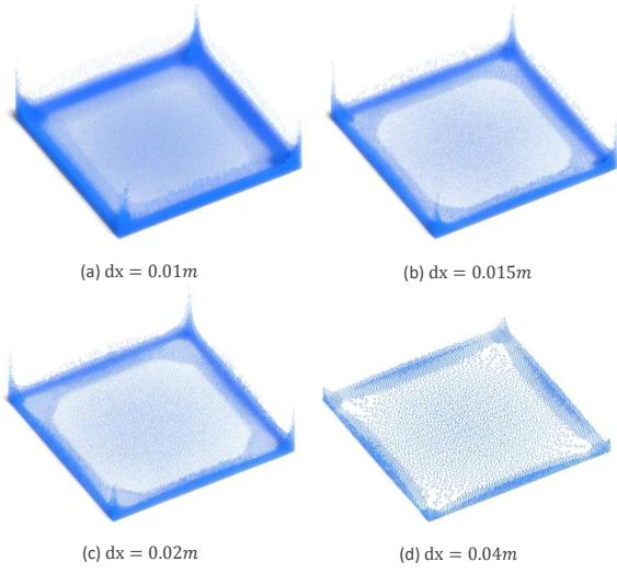
Figure 7: Simulation of a dam-break scenario with a sampling distance ranging from 0.01m, 0.015m, 0.02m to 0.04m. The time steps are all set to 0.001s, the smoothing lengths are defined as 1.2 times the particle size dx , and the gravity is 9.8m/s^2 .
